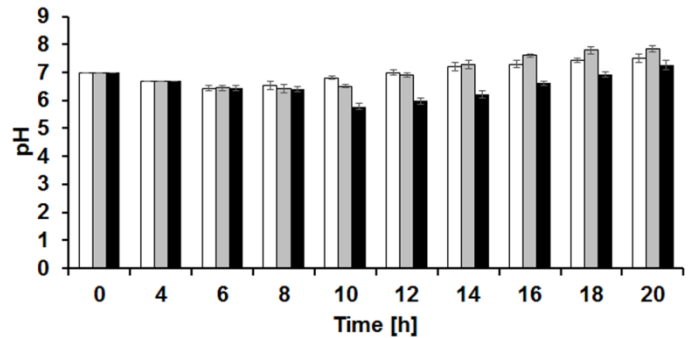
Figure 3. pH value of the growth medium in the conditions with and without the addition of phytate
