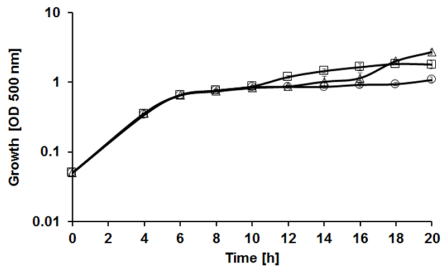
Figure 2. Growth of B. licheniformis MW3 in phosphate-starved BMM medium without and with the addition of phytate
