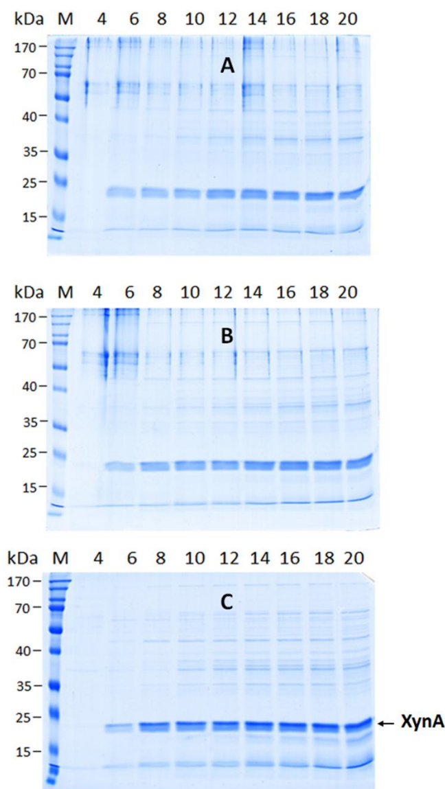
Figure 5. One-dimensional polyacrylamide gel electrophoresis separation of extracellular proteins
