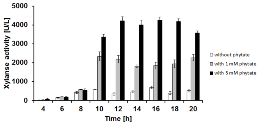
Figure 4. Xylanase activity in strain TH4 grown in the conditions with and without the addition of phytate
