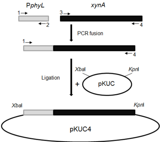
Figure 1. Schematic presentation of the cloning procedure for the construction of vector pKUC4
